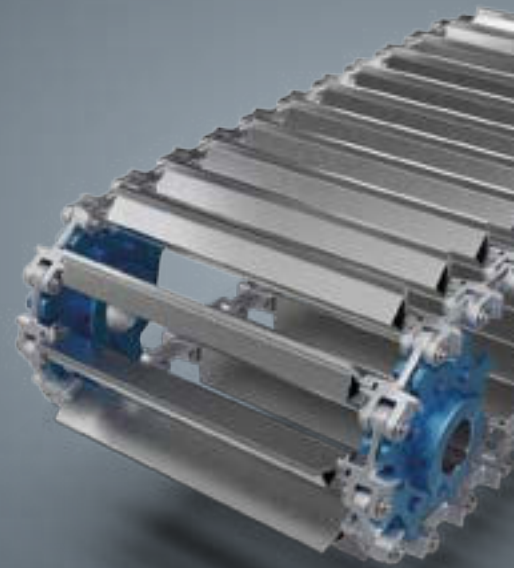
Double-strand chain. Carrier with welded reinforcement angle
